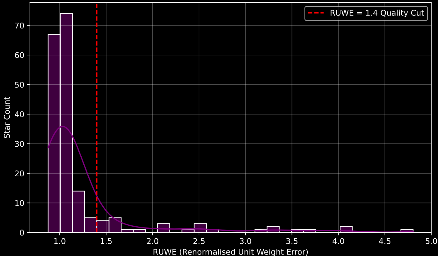
GAPOGEE DR17 Field [K2_C8_120-61_btx] RUWE Distribution (n= 187)
