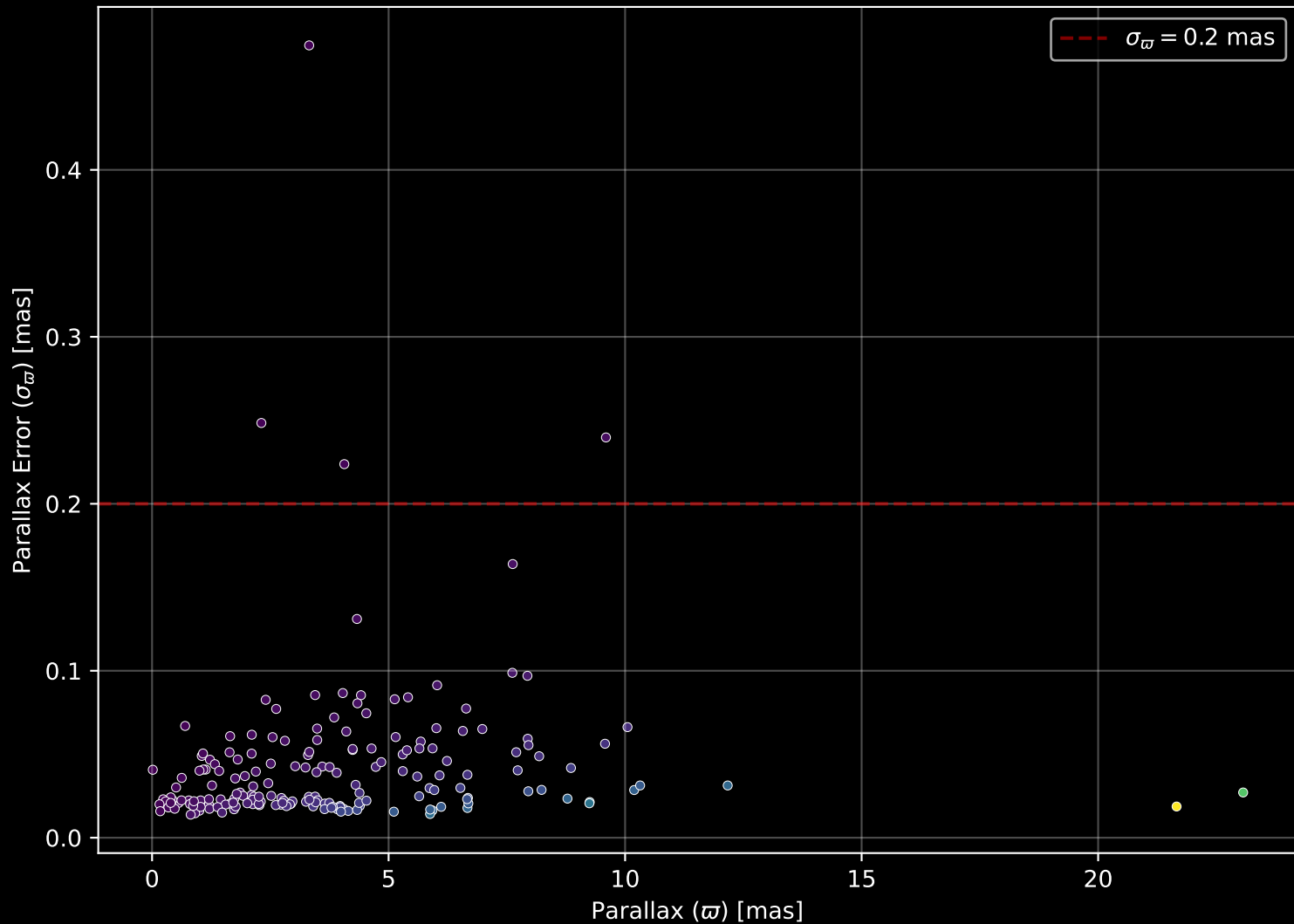
APOGEE DR17 Field: [K2_C8_120-61_btx] Parallax Quality (n= 194)
