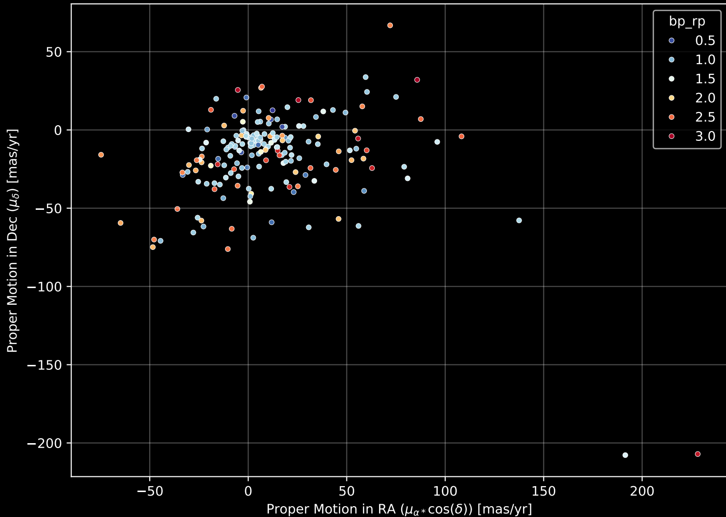
APOGEE DR17 Field: [K2_C8_120-61_btx] Proper Motion Diagram (n= 194)
