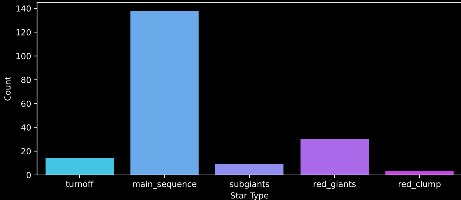
APOGEE DR17 Field: [K2_C8_120-61_btx] Count plot of Star Type
