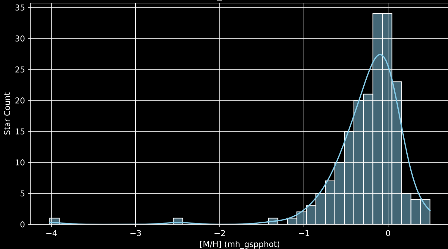
APOGEE DR17 Field: [K2_C8_120-61_btx [M/H] (mh_gspphot) (n= 191)
