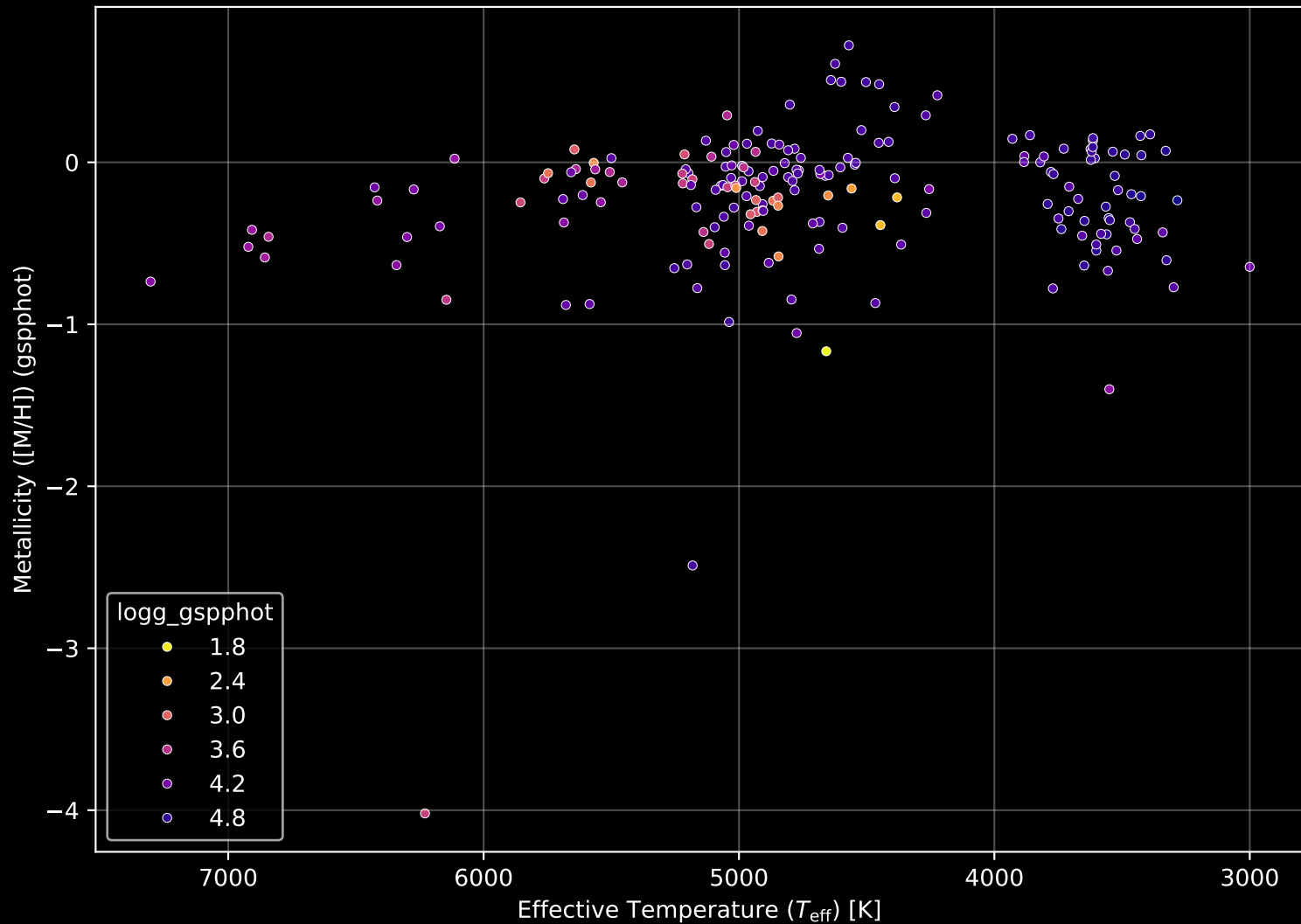
APOGEE DR17 Field: [K2_C8_120-61_btx] Stellar Population Parameters (n= 194)
